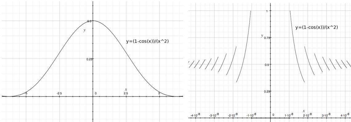
Figure 1: Graphs of Equation 1: 1a at normal zoom and 1b zoomed to the area of interest.
